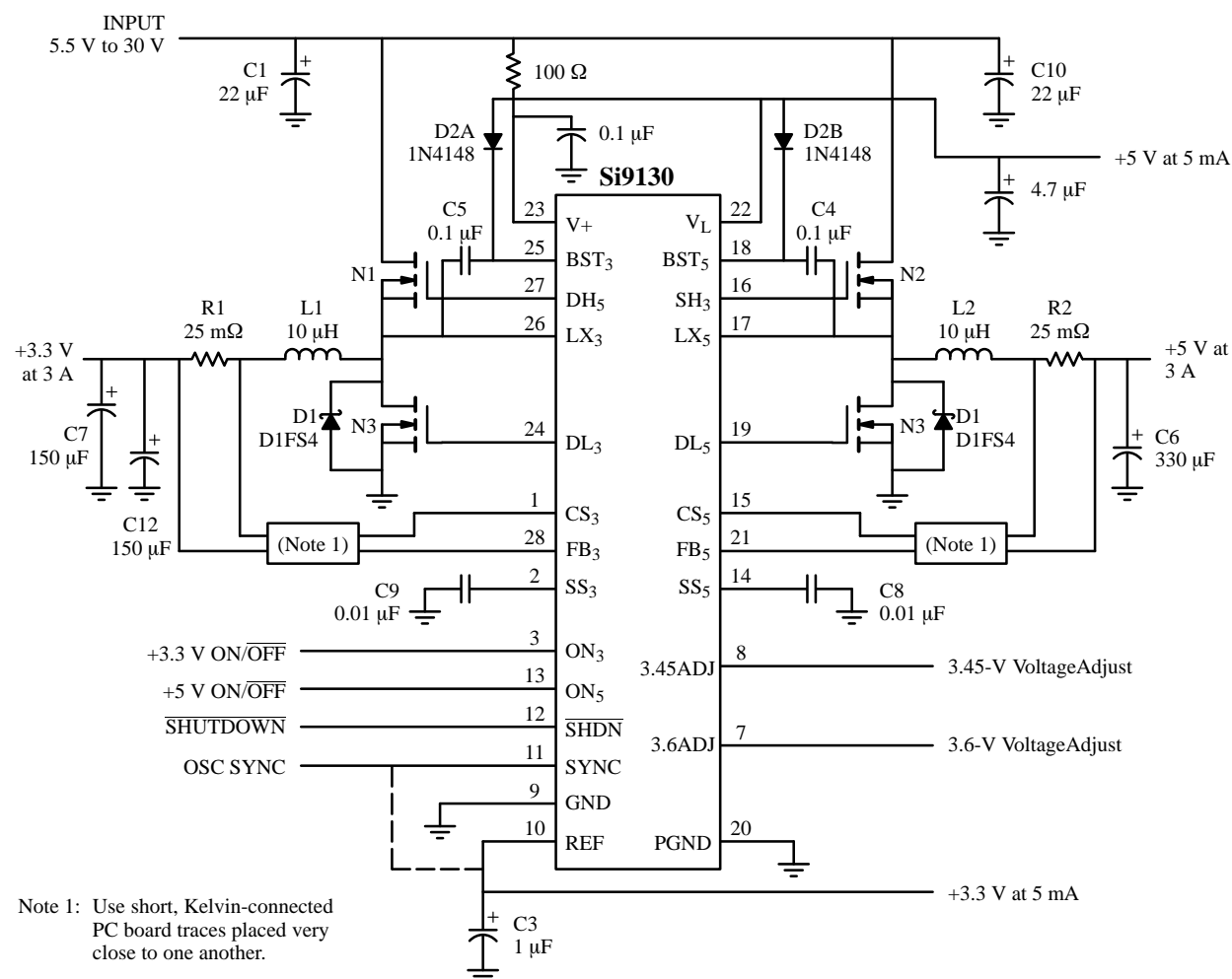
Figure 1. Si9130 Application Circuit
