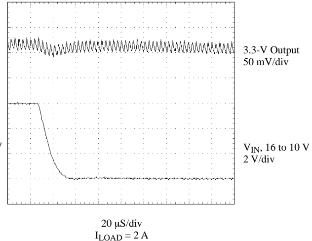
3.3-V Line-Transient Response, Falling
