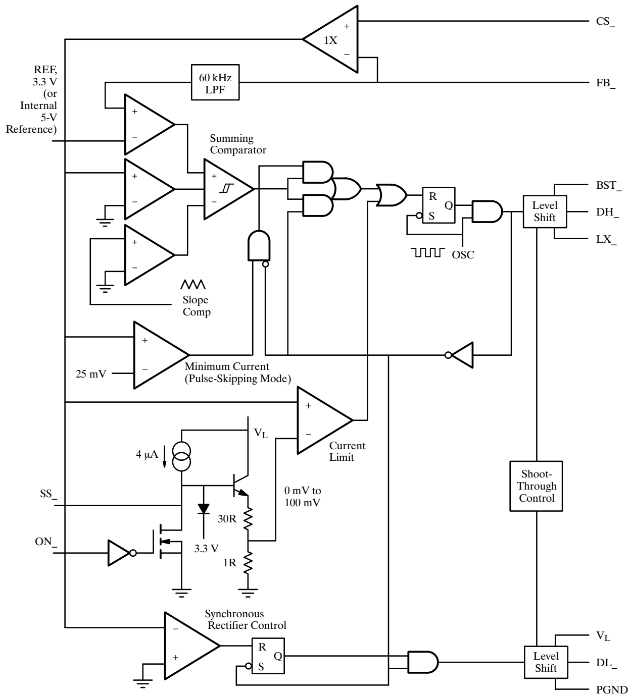
Figure 3. Si9130 Controller Block Diagram
